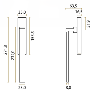
tilt-and-turn system
