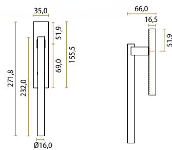
tilt-and-turn system
